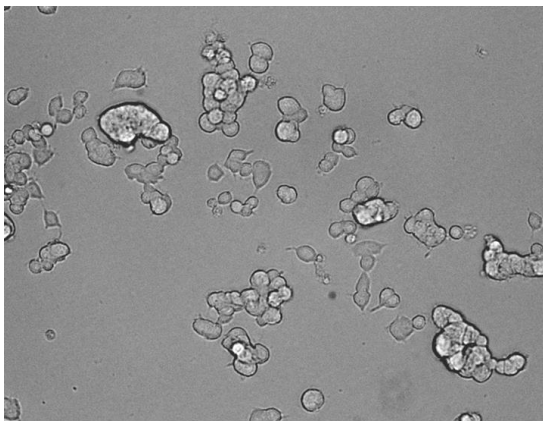
Control PC12
