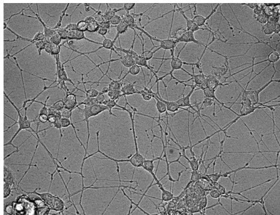
Differentiated PC12
